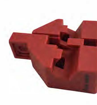
Snap on Multi Pole Breaker Lockout PS-LOTO-LCBMP
